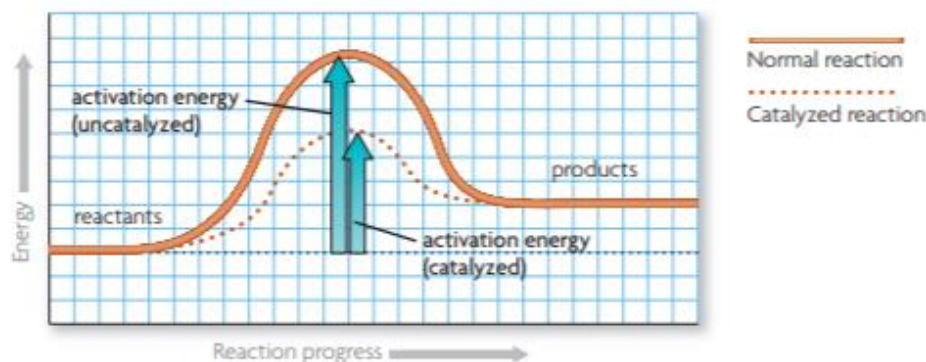
FIGURE 2.22 CATALYSTS AND ACTIVATION ENERGY
